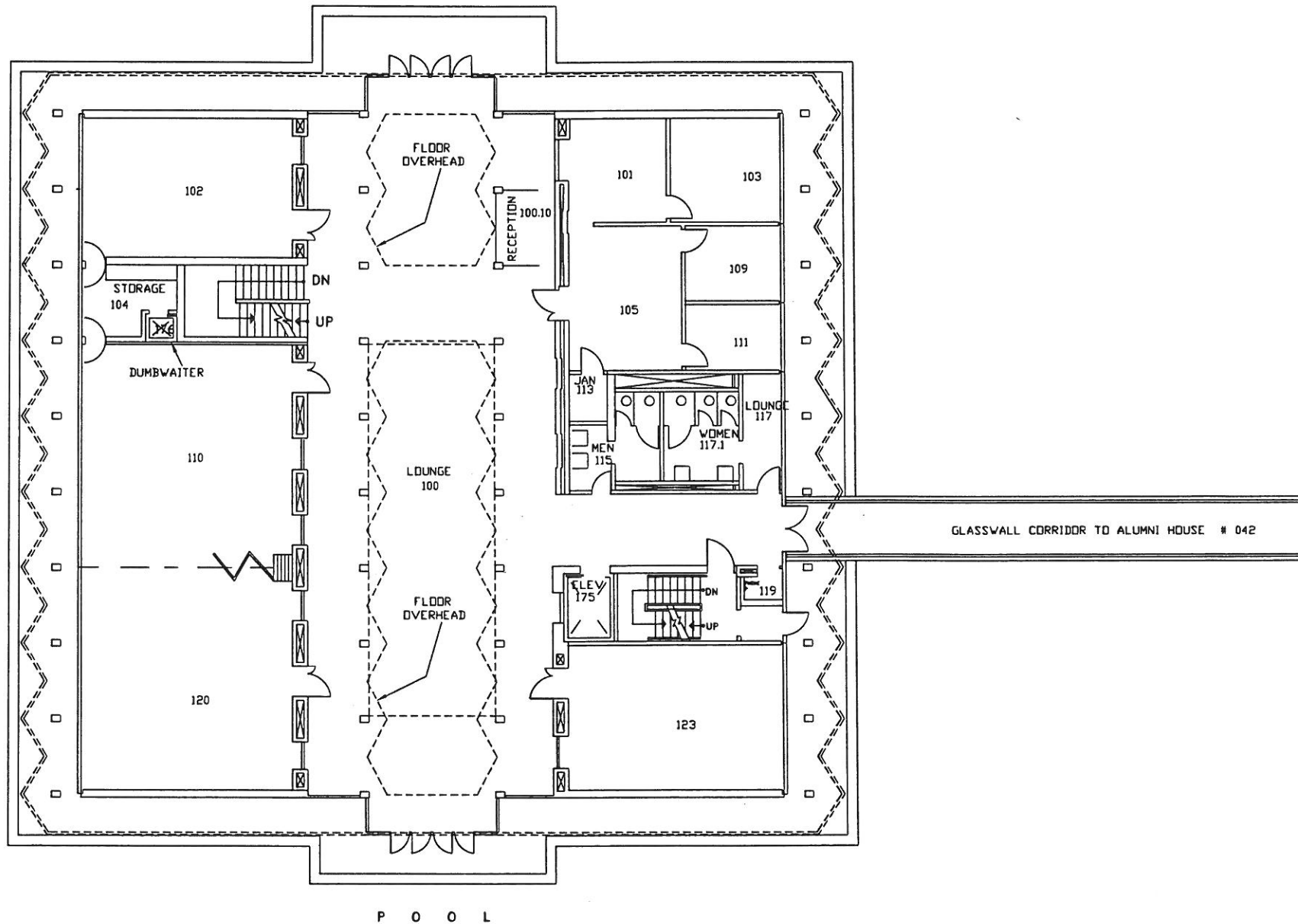
McGREGOR MEMORIAL CONFERENCE CENTER BUILDING #043 FIRST FLOOR
